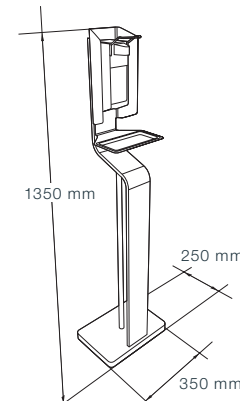
Dispenser standard EUR1 for 500 ml
